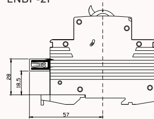
LNBF-2P
