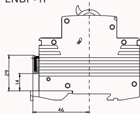
LNBF-1P
