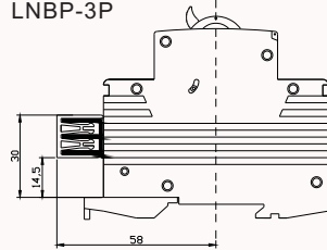
LNBP-3P
