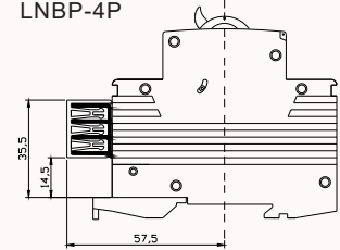
LNBP-4P
