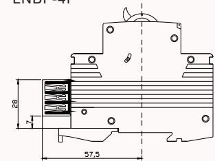
LNBF-4P
