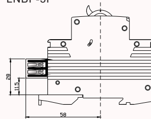
LNBF-3P
